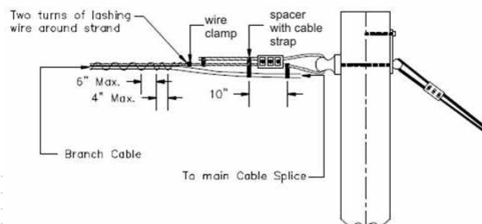
Figure 23- Typical Pole Attachment at Dead-End Pole using Moving Reel Method (RUS 1751F-635)
