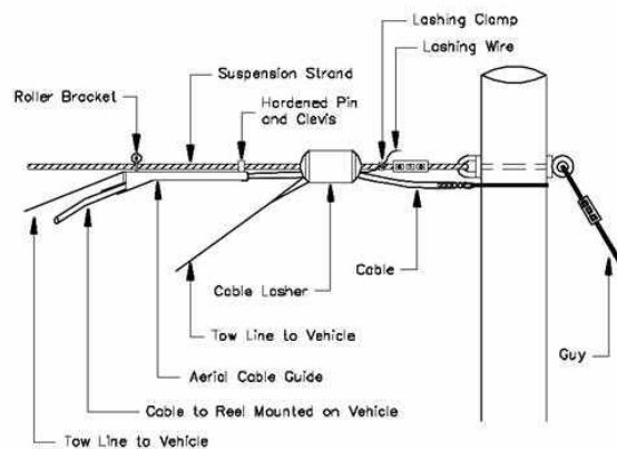
Figure 12- Start Up Configuration for Moving Reel Aerial Placement Method (RUS 1751F-635)
