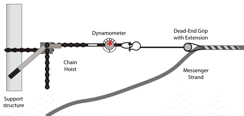
Figure 37- Tensioning of ADSS at Dead-End Support
