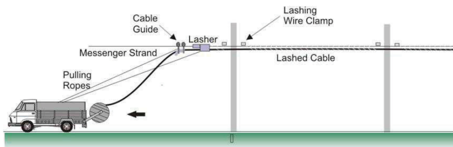
Figure 11- Schematic Drawing of the Moving Reel (Drive-Off Method) to Place Aerial Cable
