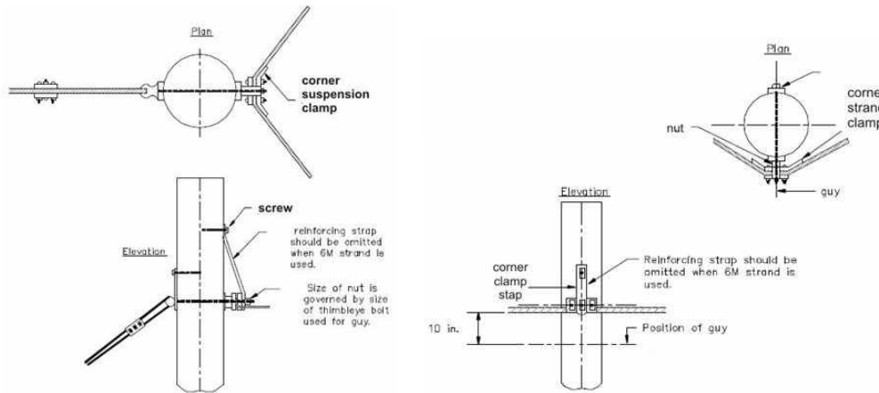
Figure 10- Corner Suspension Clamp Outside Angle 15° to 30° (left), Inside Angle (15° to 60°), (RUS 1751F-152)
