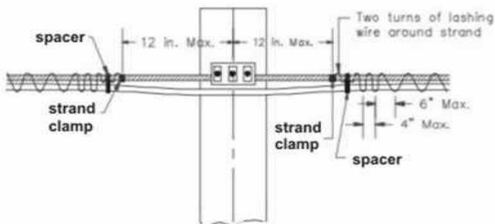
Figure 24- Intermediate Pole, Strand, and Clamp Attachment Hardware(RUS 1751F-635)
