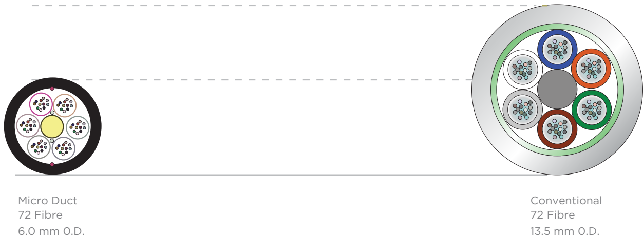
Figure 5- Comparison of STL's Micro-Duct Optical Cable to a 72 Fibre Conventional Optical Cable
