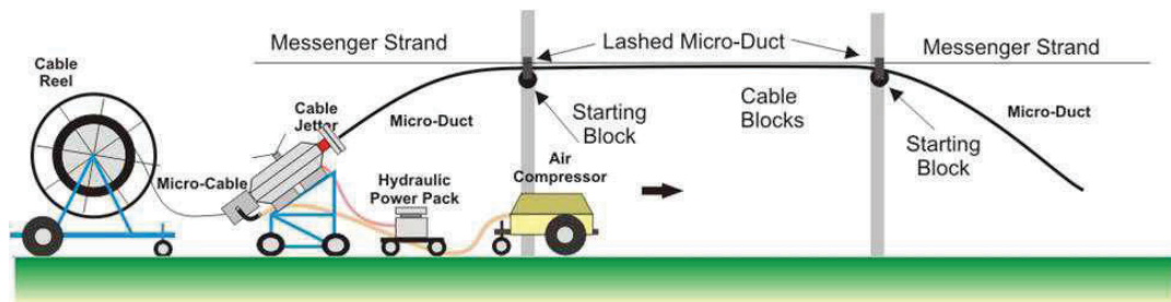
Figure 45- Cable Jetting Schematic Showing Aerial Placement in Sub-Duct Without Intermediate Assist
