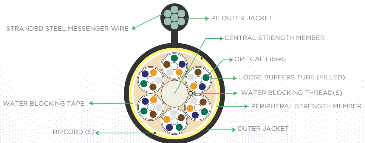
Figure 2- STL Loose Tube Figure-Eight weOight apt installilatlacnol Cable for Aerial Applications
