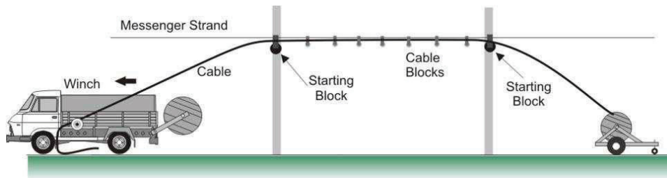
Figure 18- Stationary Reel Method, Cable Being Pulled into Cable Blocks Prior to Lashing Operation
