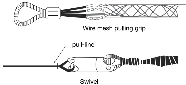
Figure 14- Pulling Hardware Required to Place Cable onto Cable Blocks During the First Stage of the Stationary Reel Placing Method
