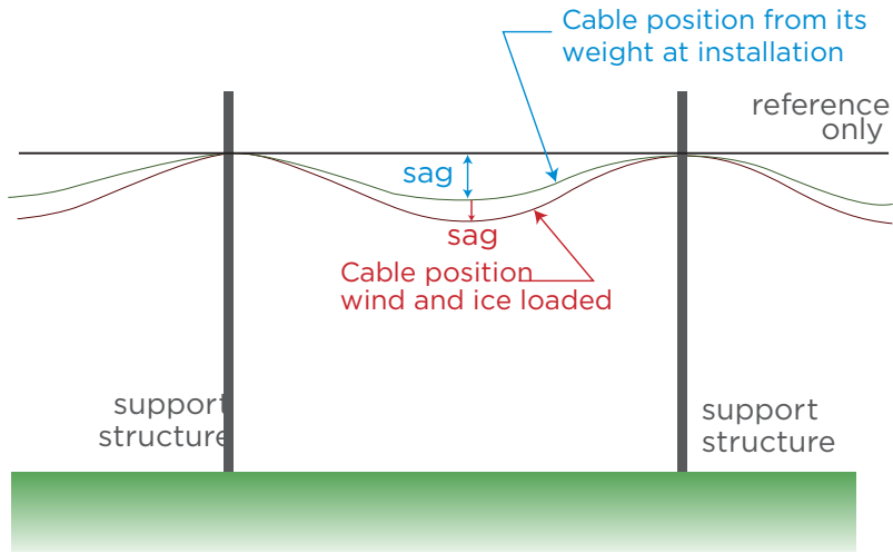
Figure 6- Sag Drawing of Aerial Plant Catenary Cable Deflection
