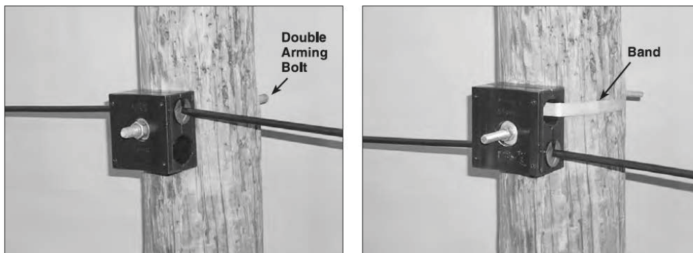
Figure 40- FibreLIGN® Lite Tangent Supports Bolt-Mounted (Left) and Band-Mounted (Right).
