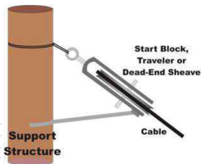
Figure 34- Supported Traveler or Sheave at Support Structure Positioned to Maintain Alignment with Cable
