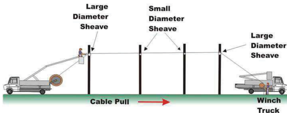
Figure 32- Stationary Reel Method: ADSS Cable Placement
