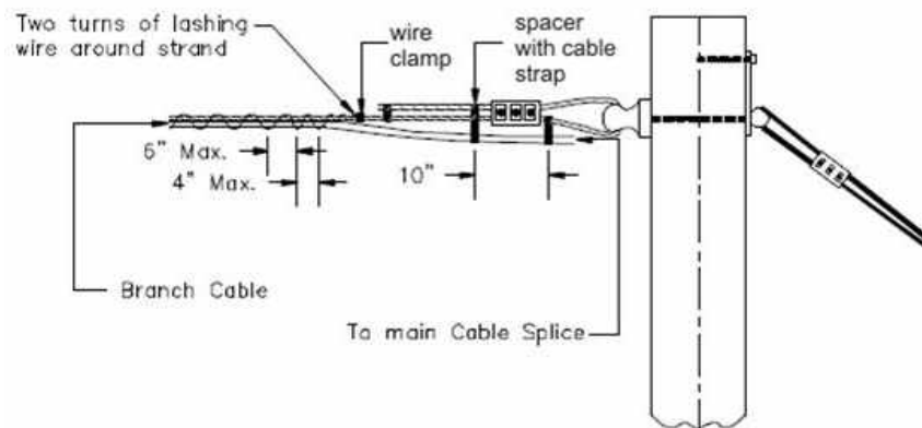
Figure 20- Pole Attachment at Dead-End Pole using Moving Reel Method (RUS 1751F-635) Place the lasher and the aerial cable guide on the messenger strand.
