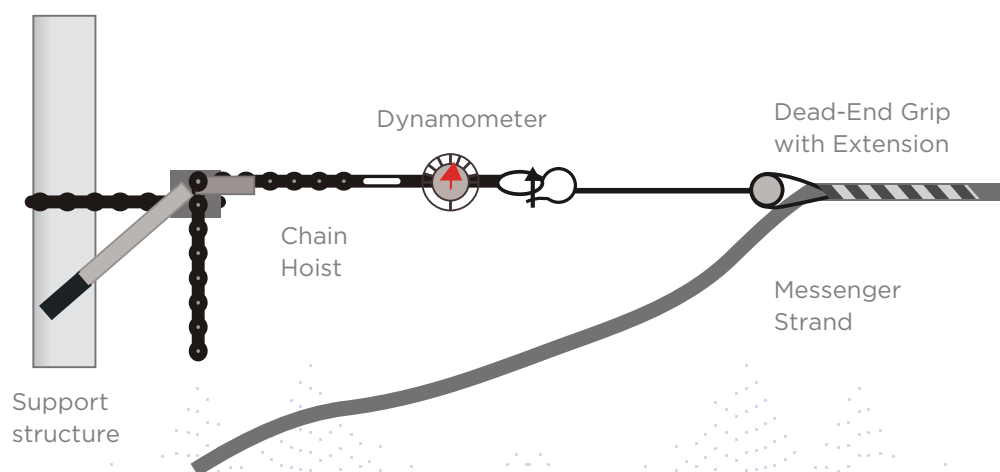
Figure 7- Tensioning the Messenger Strand Using a Dynamometer and Chain Hoist
