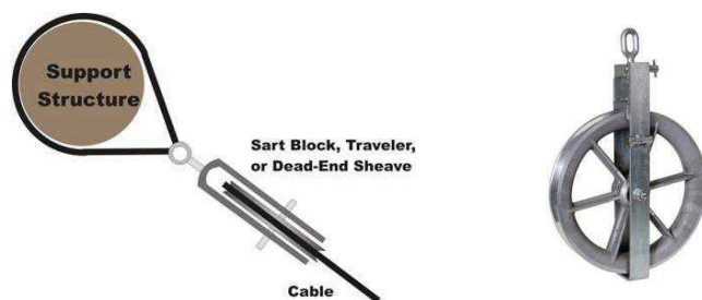
Figure 33- Supported Traveler or Large Diameter Sheave at Up-Feed and Down-Feed from Start and End Support Structures
