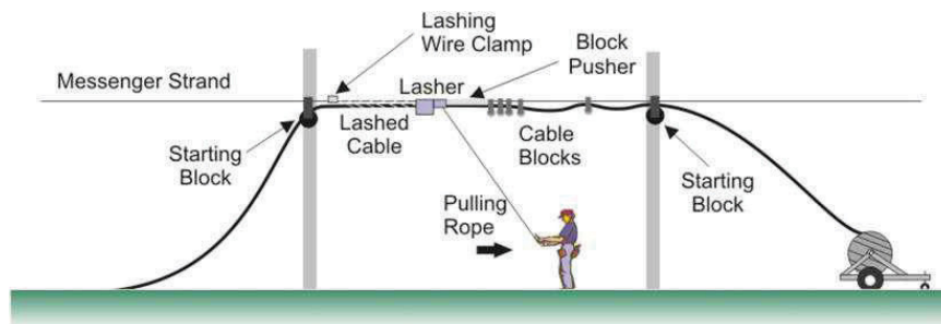
Figure 19- Stationary Reel Method Lashing Aerial Cable to Messenger Strand Being Pulled in the Opposite Direction of the Cable Placing Operation
