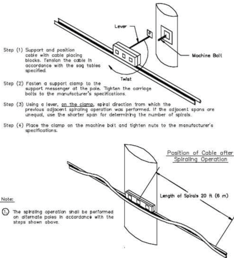
Figure 31- Spiraling Operation Detail, RUS 1753F-152
