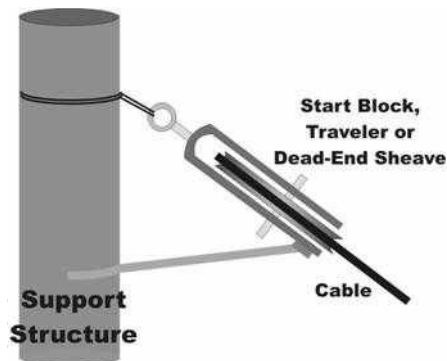
Figure 15- Starting Block for Cable Placement through Cable Blocks Used at First and Last Pole
