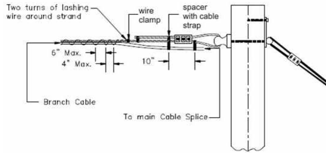
Figure 13- Typical Pole Attachment at Dead-End Pole Using Moving Reel Method (RUS 1751F-635)
