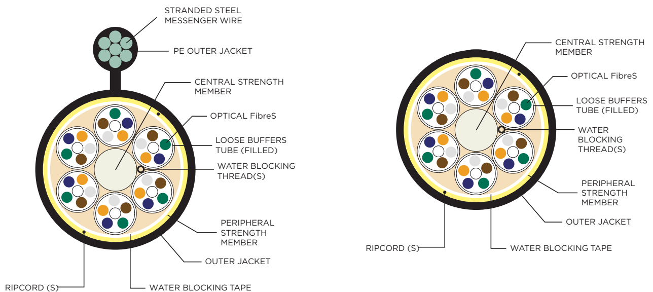
Figure 25- Two Main Self-Supporting Cables: Figure-Eight and ADSS Cables
