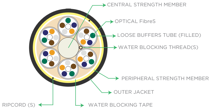
Figure 1- STL Duct-Lite™ Optical Cable for Lashed Aerial Applications
