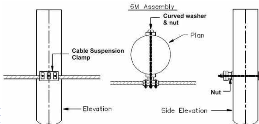
Figure 8- Suspension Cla Figure 9- Messenger Stand Pole Attachment for Cable to Pole Angles 0° to 15°; (RUS 1751F-635)mp
