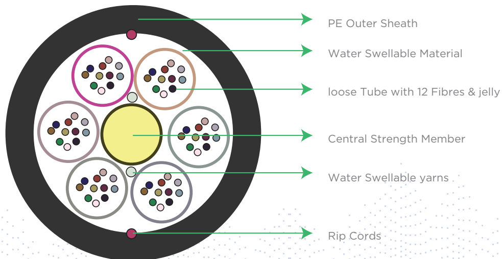
Figure 4- Cross-Section of STL's Micro DUCT-LITE™ Multitube Fibre Optic Cable
