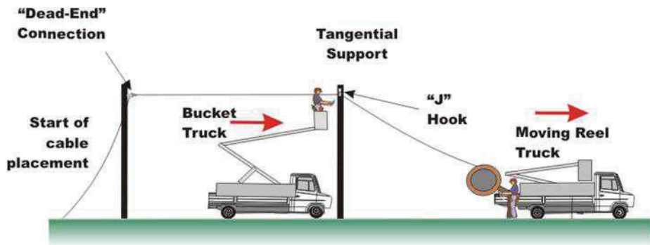
Figure 38- Moving Reel ADSS Cable Placing Method
