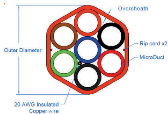
Figure 43- Multiple Micro-Duct Unit Available in Different Numbers of Sub-Ducts and Different Sizes (photograph courtesy A-D Technologies)
