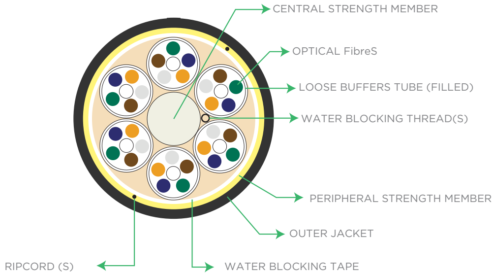
Figure 3- STL Aerial-Lite™ (ADSS) Optical Cable for Aerial Applications
