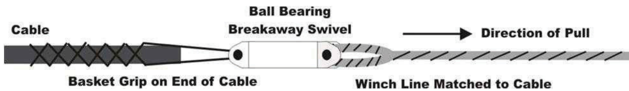
Figure 35- Cable Placement Array Using Ball-Bearing Swivel to Connect Winch Line to Cable
