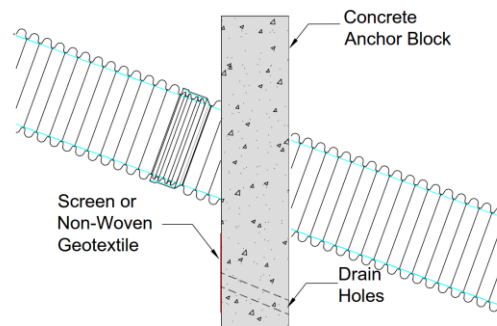
Figure 9.28: Typical Concrete Anchor Block on Steep Slopes
